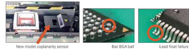
New model coplanarity sensor, Bad BGA ball, Lead float failure
